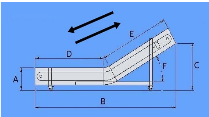
n.5 - INCLINED DOWNWARD WITH A HORIZONTAL BASE SECTION
