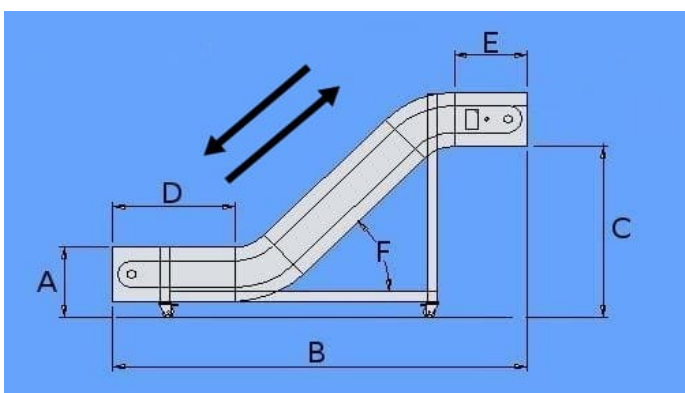
n.9 - SWAN-NECK CONVEYOR - DOWNWARD
