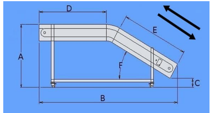
n.7 - INCLINED UPWARD WITH A HORIZONTAL BASE SECTION
